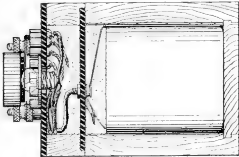
Fig. 5. Sectional view of case taken through testing-lamp
